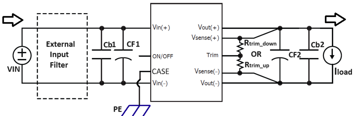
Figure-12: Typical electrical connection (Positive logic)
